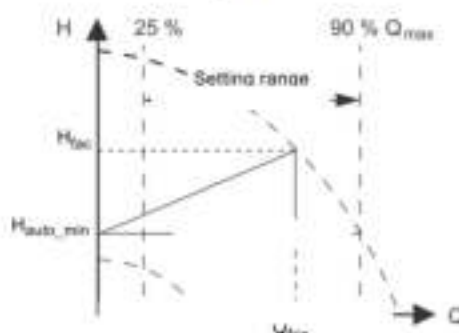
Fig. 51 FLOW ADAPT
