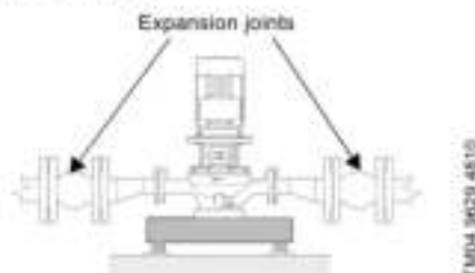
Fig. 12 TP pump installed with larger expansion joints
