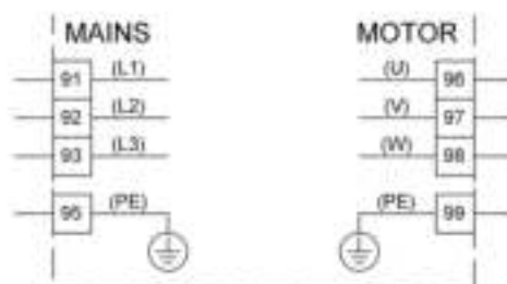
Fig. 157 Wiring diagram, three-phase
