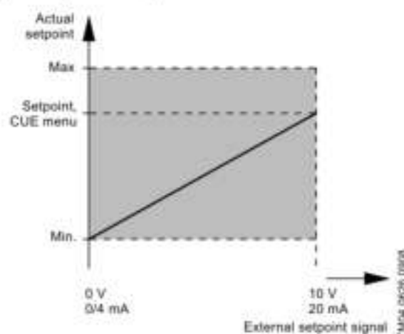
Fig. 106 External setpoint
