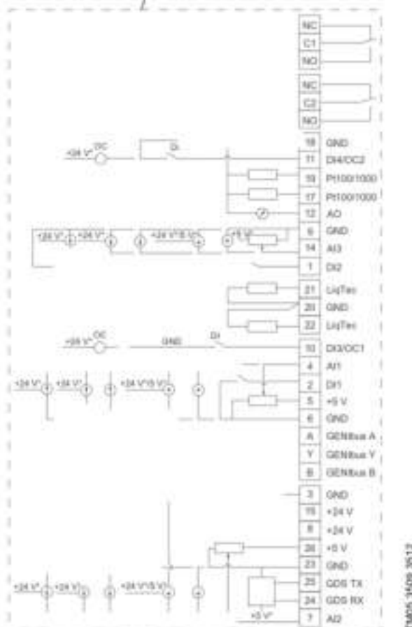
Fig. 147 Connection terminals, FM 300, option
