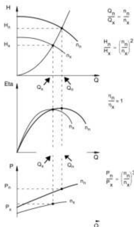
Fig. 128 Affinity equations
