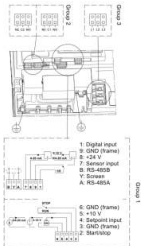
Fig. 149 Connection terminals
