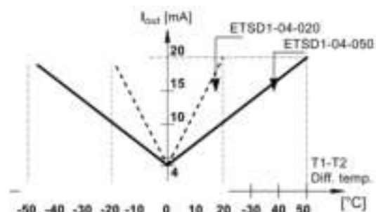
Fig. 177 Sensor characteristics
