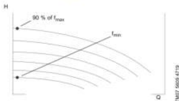
Fig. 115 QH curve for variable speed pump for choosing low flow operating points
