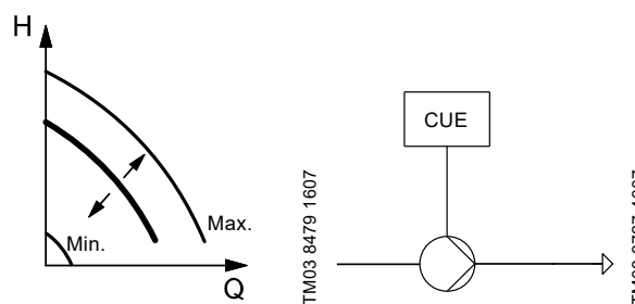
Fig. 88 Open loop, constant curve
