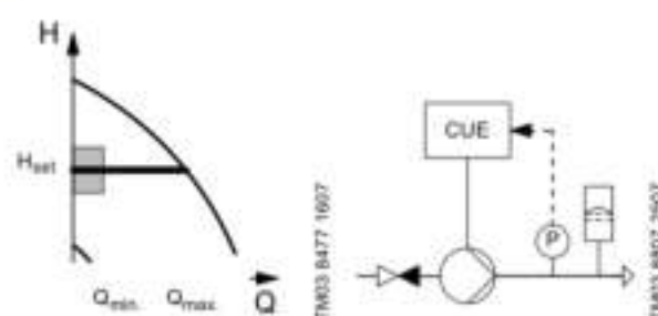
Fig. 90 Constant pressure with stop function
