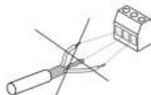
Fig. 154 Do not twist the screen ends
