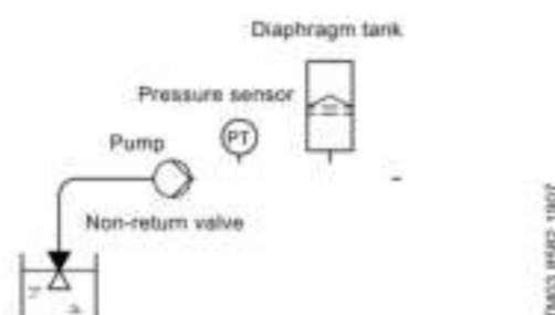
Fig. 92 Position of the non-return valve and pressure sensor in a system with suction lift
