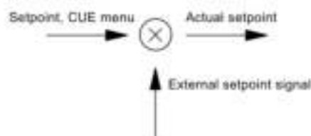
Fig. 105 Setpoint, CUE menu and external setpoint signal
