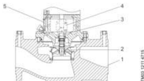
Fig. 12 Sectional drawing of TP Series 200 with flange connection
