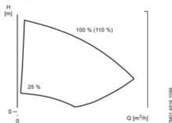
Fig. 20 Duty range of TPE Series 2000 pumps
