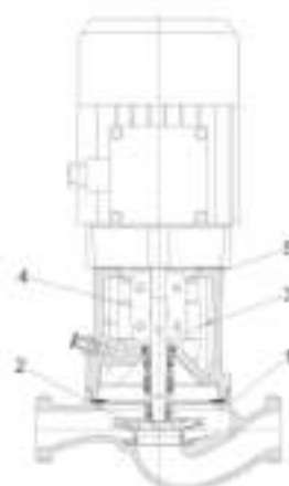
Fig. 11 Sectional drawing of TP Series 100 with union connection
