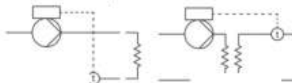
Fig. 57 "Constant temperature"
