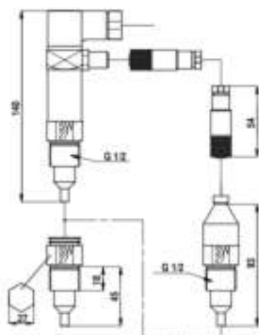
Fig. 178 Dimensional sketch
