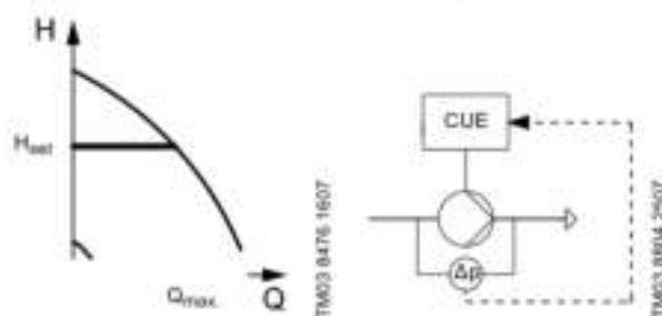
Fig. 94 Constant differential pressure, pump
