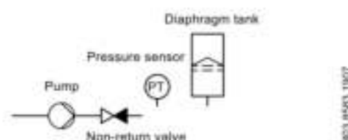
Fig. 93 Position of the non-return valve and pressure sensor in a system with positive inlet pressure
