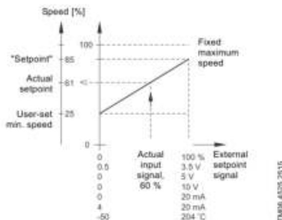
Fig. 76 Example of setpoint influence with constant curve
