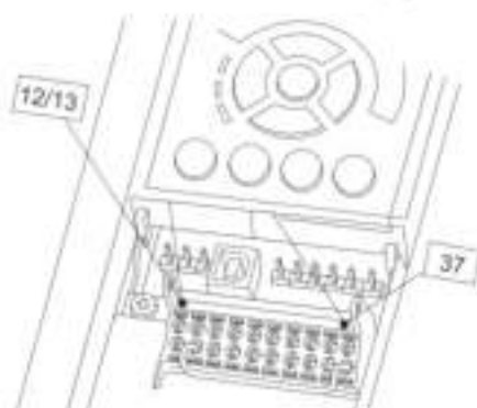
Fig. 161 Remove jumper
