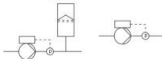
Fig. 55 "Constant pressure"
