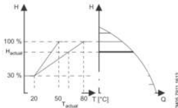
Fig. 81 "Temperature influence"
