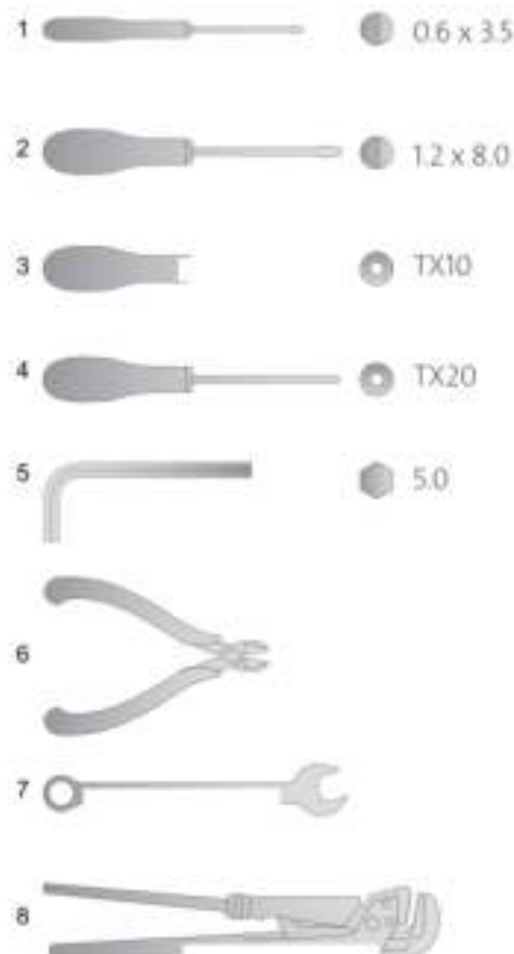
Fig. 7 Recommended tools
