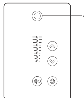
Fig. 8 Control panel
