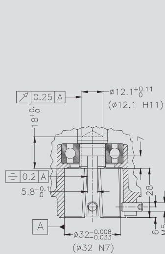
DETAIL C Scale 3/2
